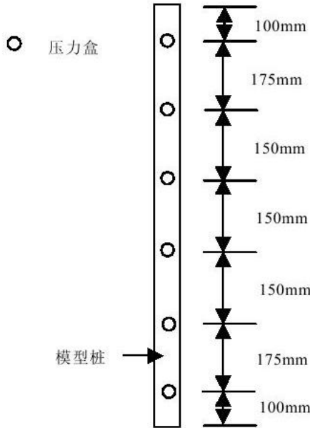
Fig. 1 Model test layout
